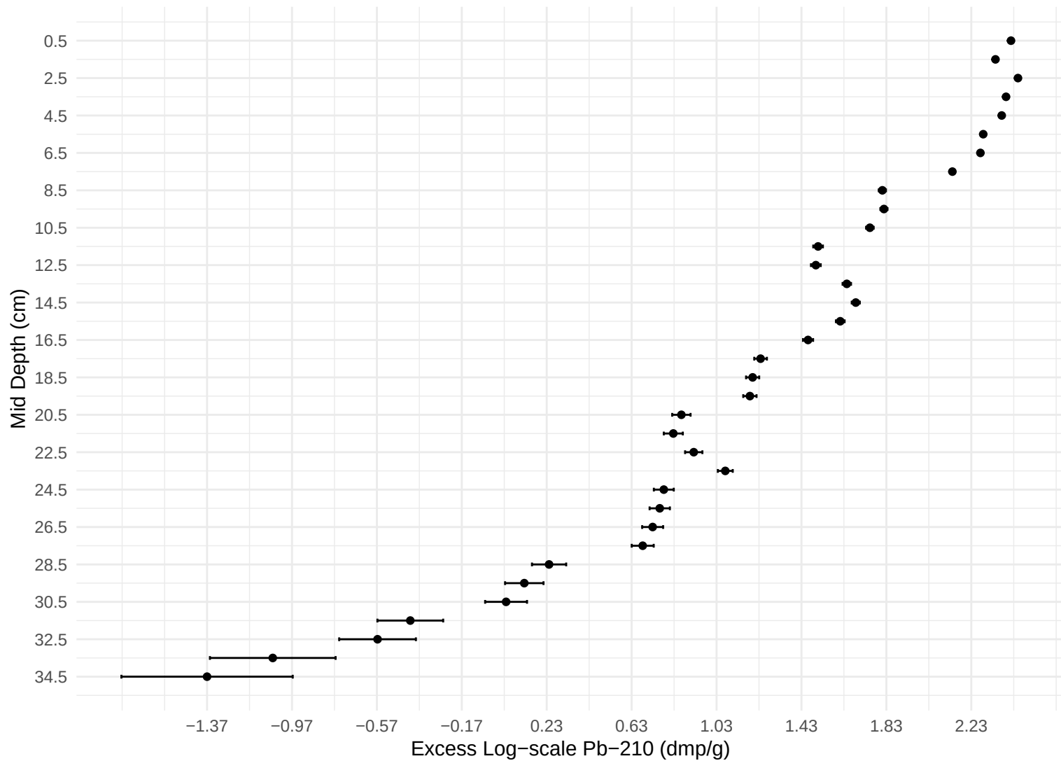
Excess Log-scale Pb-210 vs Depth
